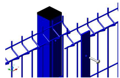
RFS Steel Clamp Bar Fixing
