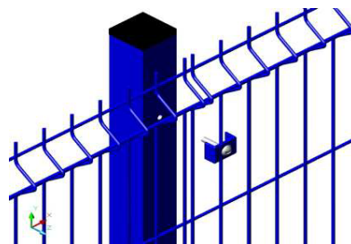
RFS Cal-Tech Steel Clip Fixing
